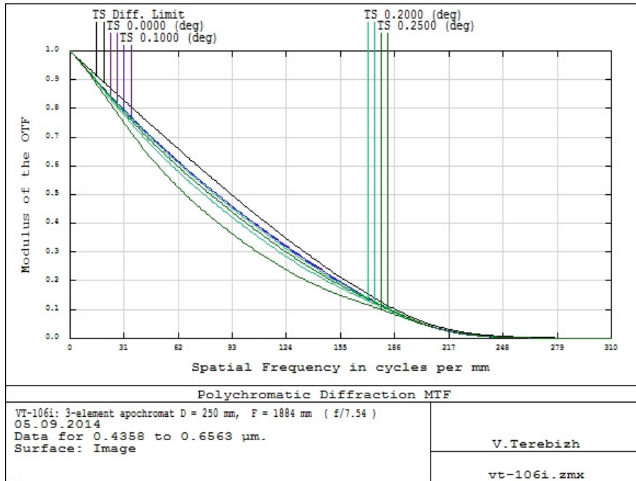
Modulation Transfer Function in polychromatic waveband 0.4358 – 0.6563 μm for the field angles 0 – 0.25°
