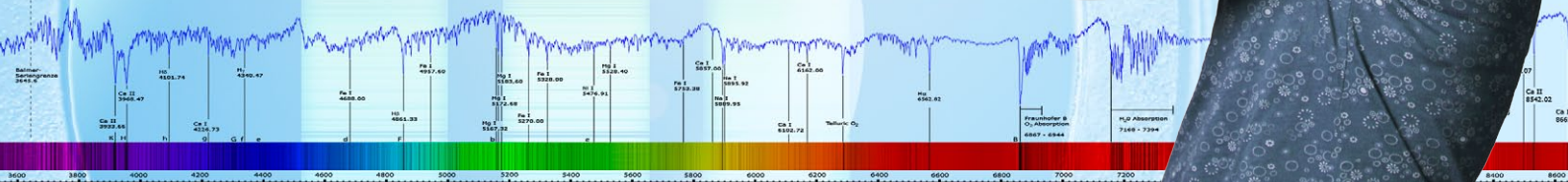
The Solar Spectrum
